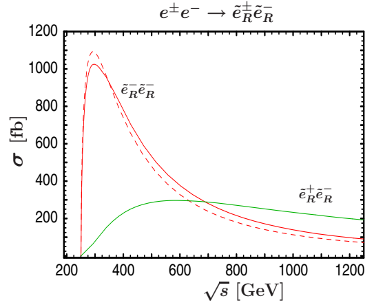
Fig. 5. Total cross sections for smuon and selectron pair production in e^\pm e^- annihilation [74]. The Born cross section (broken lines) is shown for comparison
