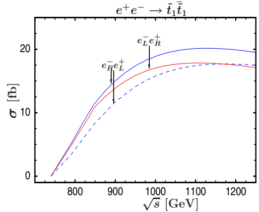
Fig. 6. Total cross sections for \tilde{t}_1 \bar{\tilde{t}}_1 pair production in e^+e^- annihilation for left- and right-handed polarized electron ( P_{e^-} = 0.8 ) and positron ( P_{e^+} = 0.6 ) beams [75]. The Born cross section (broken line) is shown for comparison
