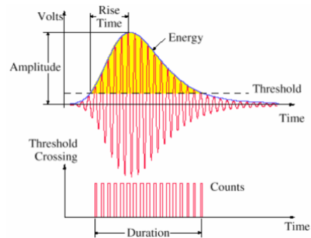
Fig.1. Acoustic emission feature [15]
