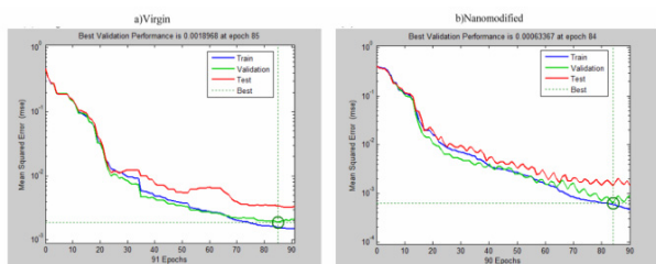
Fig.6. Performance plot: (a) Virgin and (b) Nanomodified
