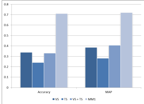
Figure 1. Performance comparison of MM1 and baseline in terms of accuracy and MAP.
