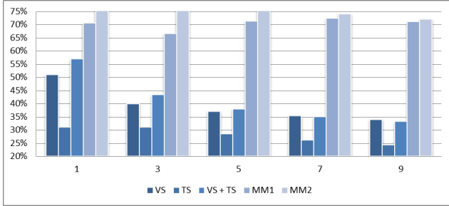
Figure 2. Systems' accuracy comparisons according to different k number of retrieved images for each query.
