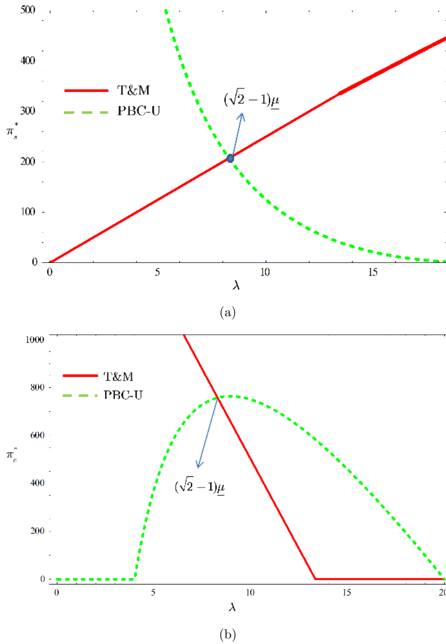
FIGURE 4.2: The supplier's (a) and the customer's (b) optimal profit under T&M and PBC-U. r = 2000, c = 1, \underline{\mu} = 20, \gamma_s = 0.01 .
