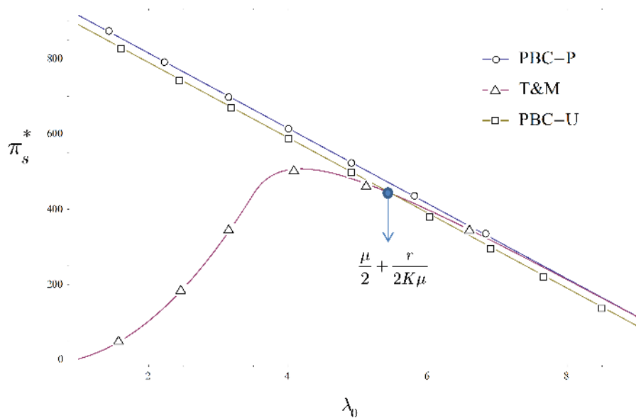
FIGURE 4.4: The supplier's profit at equilibrium under contracts, exogenous \mu . r = 1000, K = 100, \mu = 10 .
