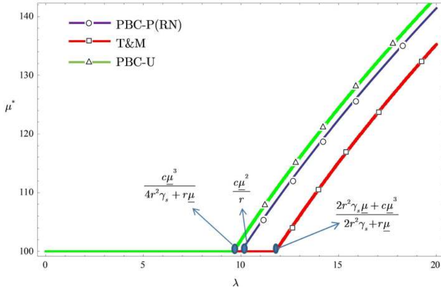
FIGURE 4.1: Optimal service capacity under risk aversion. r = 1000, c = 1, \underline{\mu} = 100, \gamma_s = 0.001 .
