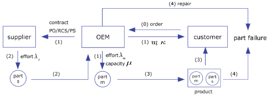
FIGURE 3.1: Sequence of events.
