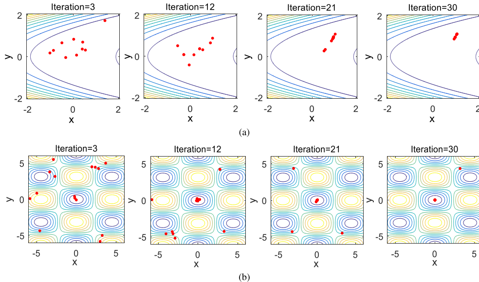
FIGURE 7. Swarm search of SDO in a two-dimensional space. (a) Unimodal function (Rosenbrock). (b) Multimodal function (Griewank).
