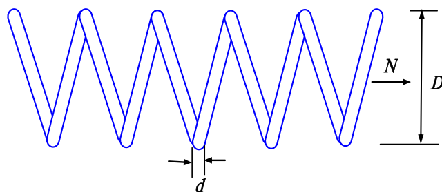
FIGURE 17. Tension/compression spring design problem.
