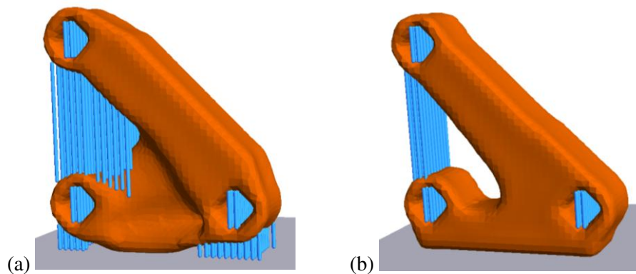
Figure 20: Optimized three-hole bracket. (a) Unconstrained (b) Constrained with h = 0.50 .
