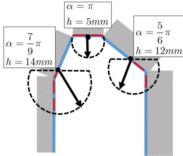
Figure 7: Searching for self-supporting boundary.
