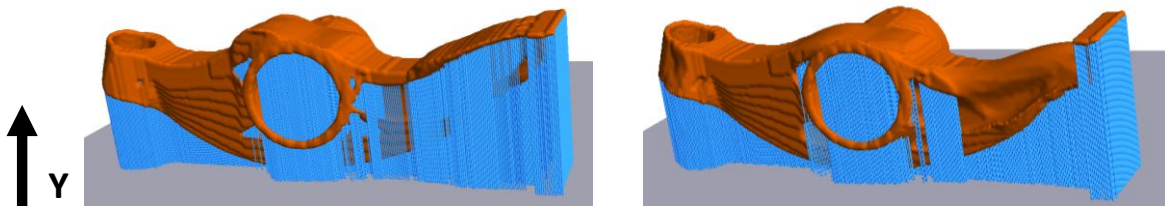
Figure 28: Build direction along +Y direction: (a) unconstrained, and (b) constrained.
