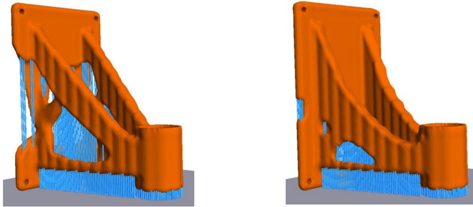
Figure 22: Optimized mount bracket at 0.7 volume fraction. (a) Unconstrained (b) h = 0.80 .
