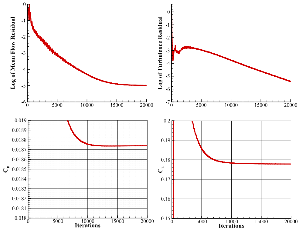
Figure 11. Without support system convergence history, M_\infty=0.85 , \alpha=0.0^\circ , Re_c=5 million.
