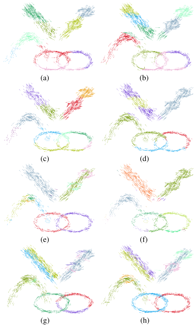
Fig. 7. Clustering results of the methods used for comparison on the synthetic data set. Colors represent the affiliation to the clusters. The SVMC is the only method that correctly estimates all the motion clusters. The resolution of each image is 467 \times 366 . (a) N-CUT. (b) K-AP. (c) MS. (d) StrAP. (e) IDPMM. (f) SVC. (g) CF. (h) SVMC.
