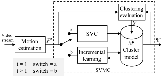
Fig. 1. Block diagram of the proposed approach. We first estimate the cluster boundaries and then use a Quasiconformal Kernel Transformation along with the online performance evaluation to refine the cluster boundaries. Then, we label each cluster and assign these labels to the respective feature vectors. M^t defines the cluster model at a generic time t , \Psi^t is the set of clusters, and S^t is the dissimilarity score that quantifies the clustering performance. SVC: support vector clustering. SVMC: support vector motion clustering.
