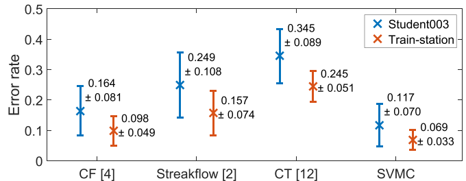
Fig. 12. Comparison of motion clustering error rates on Student003 and Train-station . SVMC outperformed CF, Streakflow, and CT in terms of number of correctly clustered people (i.e., lower error rate) for both videos.
