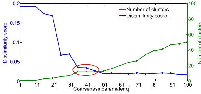
Fig. 3. Dissimilarity score and number of clusters as a function of q^t . The red ellipse shows the range of q^t values in the case of a constant number of clusters. Within this interval, we select the value of q^t corresponding to the smallest dissimilarity score.
