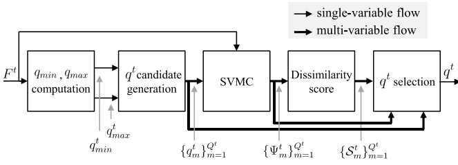
Fig. 4. Iterative process for the automatic generation of the coarseness parameter q^t using the input features F^t . SVMC: support vector motion clustering.
