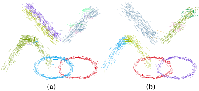
Fig. 8. Comparison of the results of (a) SVMC and (b) IDPMM at frame 22 of the synthetic data set. Some feature vectors of the two small circular flows (top-right) are incorrectly assigned to different clusters by SVMC whereas IDPMM correctly clusters them. The resolution of each image is 467 \times 366 .
