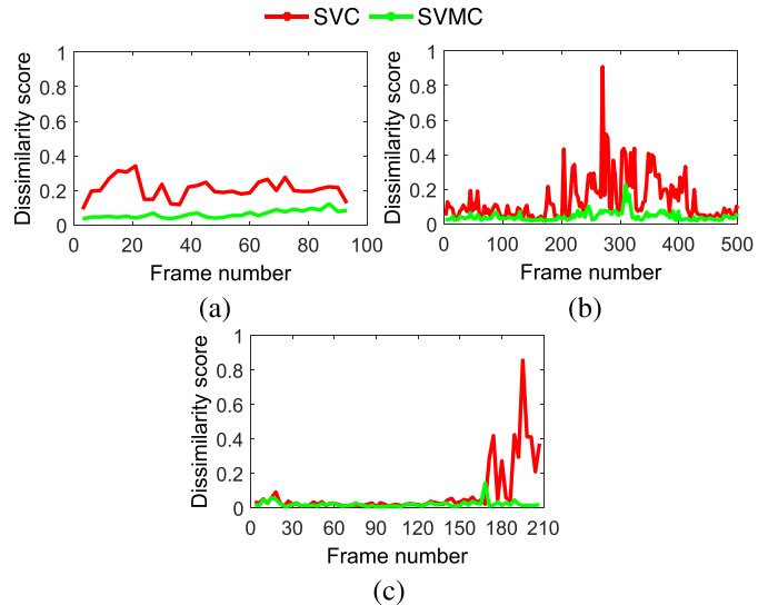
Fig. 9. Comparison of the dissimilarity scores generated by SVMC and SVC for (a) Train-station , (b) Student003 , and (c) Cross-walk . SVMC (green) produces clusters with feature vectors that are more coherent (i.e., lower dissimilarity score) than SVC (red).
