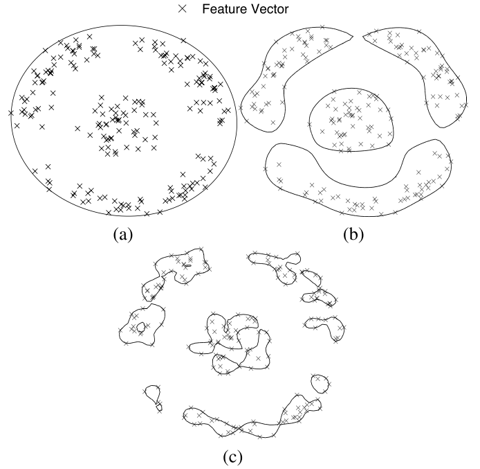
Fig. 2. Example showing three different clustering steps with (a) q^t, q_{\min}^t = 0.2 , (b) q = 10 , and (c) q = 25 . Only one cluster is generated when q^t, q_{\min}^t , and the number of clusters increases when the value of q increases.
