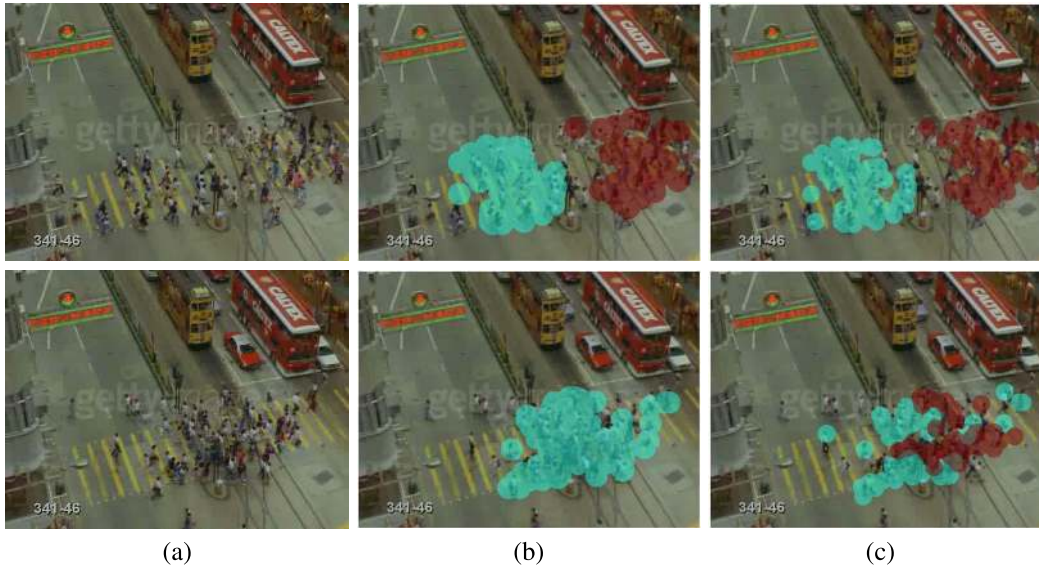
Fig. 11. Sample clustering results on (a) representative frame of Cross-walk for (b) SVC and (c) SVMC. The colored patches represent the motion clusters of people with the same motion direction. At the 50th frame (top), both SVMC and SVC correctly cluster the two sets of people; at the 150th frame (bottom), the SVC incorrectly clusters the two sets of people as one large cluster (cyan patch). SVMC can correctly cluster the two groups of intersecting people (i.e., cyan and dark red patches).
