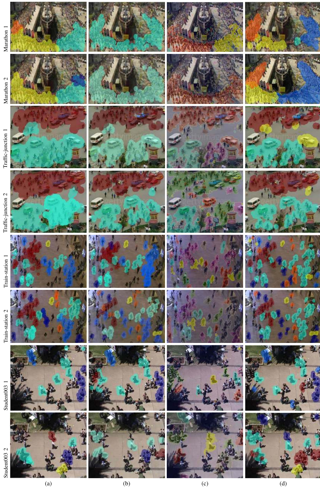
Fig. 13. Comparison of the crowd motion clustering results on different frames. Color patches represent motion clusters with the same motion direction. (a) CT [12]. (b) CF [4]. (c) Streakflow [2]. (d) SVMC.
