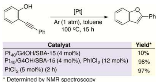
Figure 4. Hydroalkoxylation reaction with Pt catalysts.
