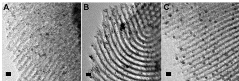
Figure 2. Representative TEM images of DEMCs supported in SBA-15. Rh 40 /G4OH/SBA-15 (A), Pt 40 /G4OH/SBA-15 (B), and Au 40 /G4OH/SBA-15 (C). Scale bars are 10 nm.
