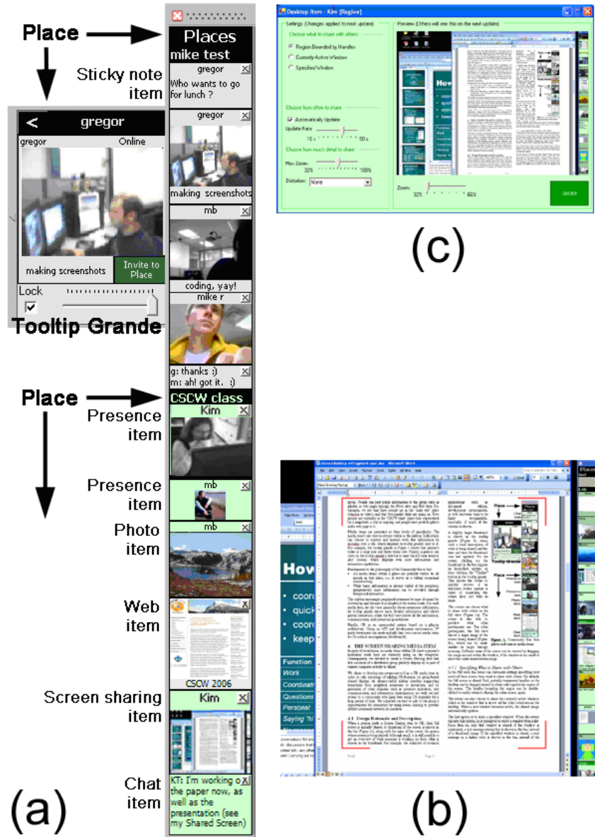
Figure 3: Community Bar and the Shared Desktop Media Item. (a) Community Bar; the tile view of the shared desktop screen-sharing item is 2 nd from the bottom. (b) Full view for the person sharing their screen. (c) The region of the screen being captured is marked by adjustable semi-transparent red handles. (b) and (c) are shown scaled down in this image.
