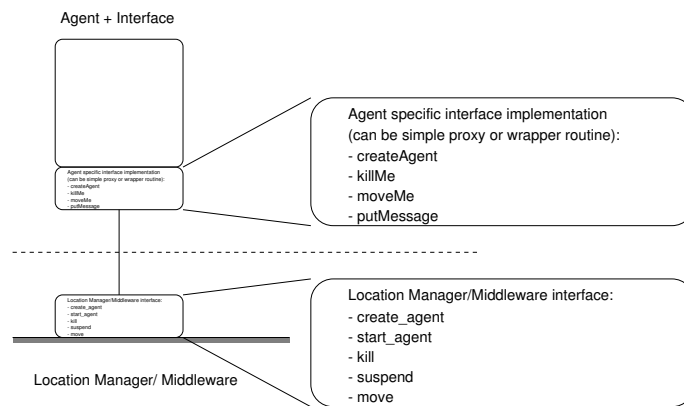
Fig. 2. The AgentScape model from the perspective of agents.
