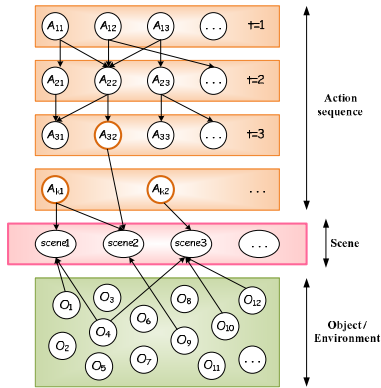
Fig 7. The action sequence represented as DBN
