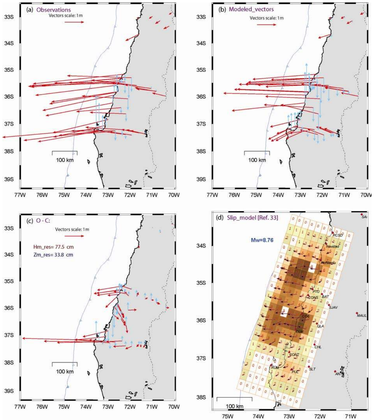
Fig. S6 Observed and computed displacement of the February 27, 2010 M_w = 8.8 Maule Earthquake, on the GPS stations from the finite-fault slip distribution of G. Hayes 33 . Observed horizontal (red) and vertical (blue) displacement vectors on the GPS networks of the Central South area of Chile (cGPS and repetition French-Chilean GPS network)
