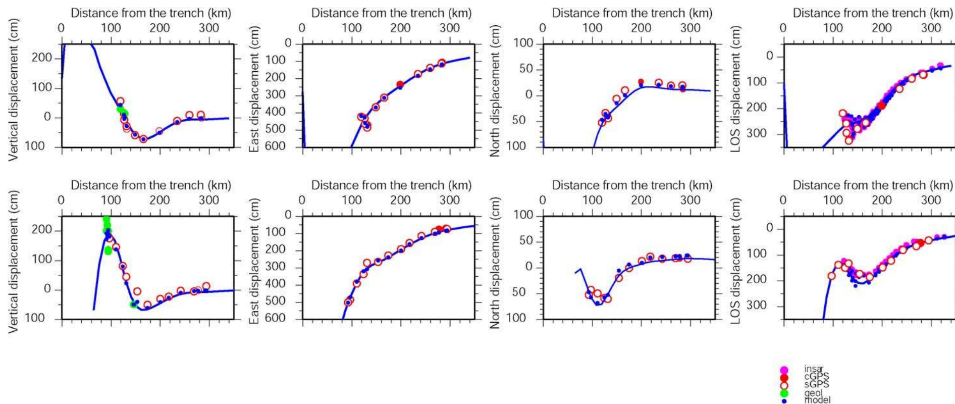
Fig. S1 Cross section of displacements against distance to trench. The two cross sections correspond to the two dashed lines on Fig. 3, approximately at the latitudes of Constitucion (upper boxes) and Arauco-Concepcion (lower boxes). Data points located within 20km-width stripes centered on each profile are projected in the section plane. Different columns depict different projections of the displacements: uplift or subsidence (1 st column), East-West (2 nd column), North-South (3 rd column) and total displacements projected in the radar line of sight (LOS) (i.e. value of digitized SAR interferogram superimposed with 3D GPS displacements projected in the satellite LOS). Green dots show relative land-level changes measured from geological markers. Red dots show GPS measurements (full for cGPS and open for sGPS). Purple dots depict InSAR deformation. Blue dots show the value of the model at the data points, and the blue line depicts the value of the model along the cross section.
