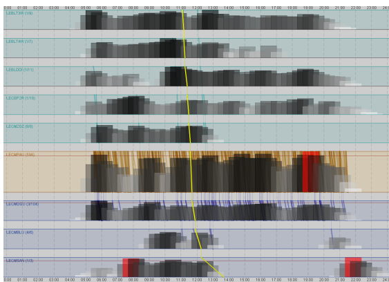
Figure 6. A timetable view in the mode of showing the full path of one selected job through the machines serving it. In this example, it is the job highlighted in Figure 5.
