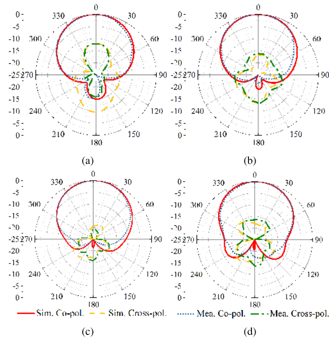
FIGURE 17. Normalized radiation patterns in the horizontal plane of the +45^\circ radiation of the LB element at (a) 0.7 GHz, (b) 0.8 GHz, (c) 0.9 GHz, (d) 0.96 GHz.
