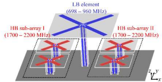
FIGURE 1. Configuration of a dual-band base station antenna array section.
