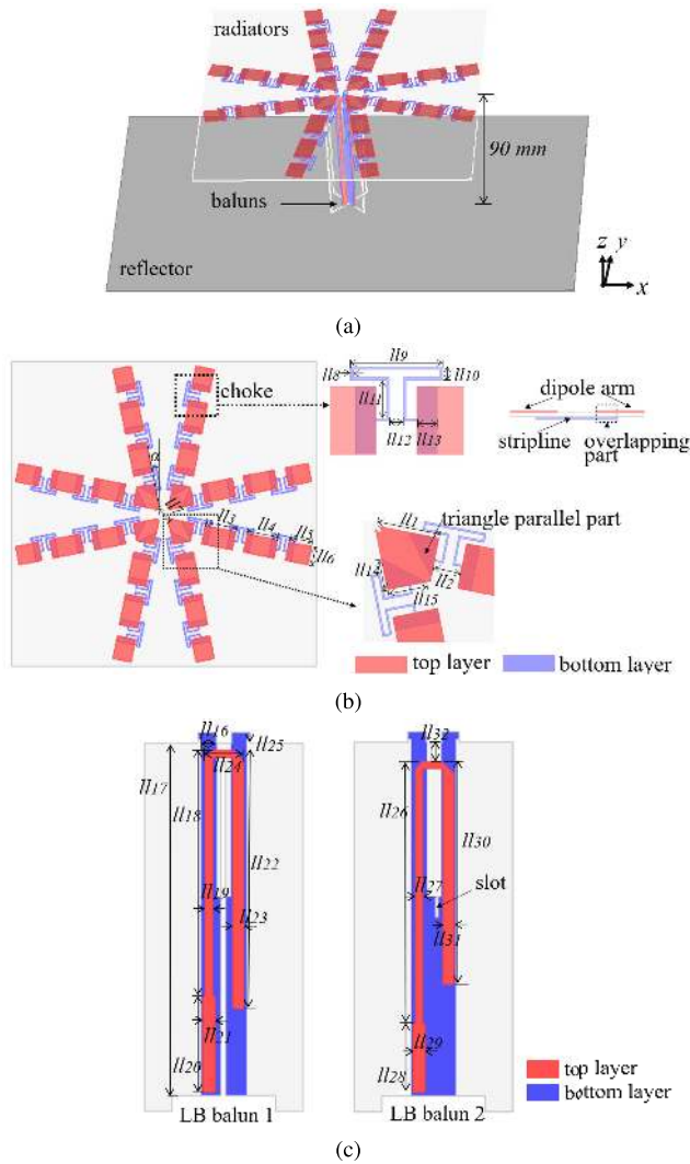
FIGURE 11. Configuration of the double-arm choked LB element: (a) perspective view of the LB element, (b) the view of the radiator, and (c) the views of baluns.
