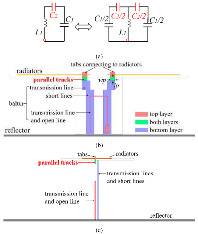
FIGURE 4. (a) Circuit model of the capacitance-loaded HB element. (b) Front view, and (c) side view of the realized capacitance-loaded HB element.
