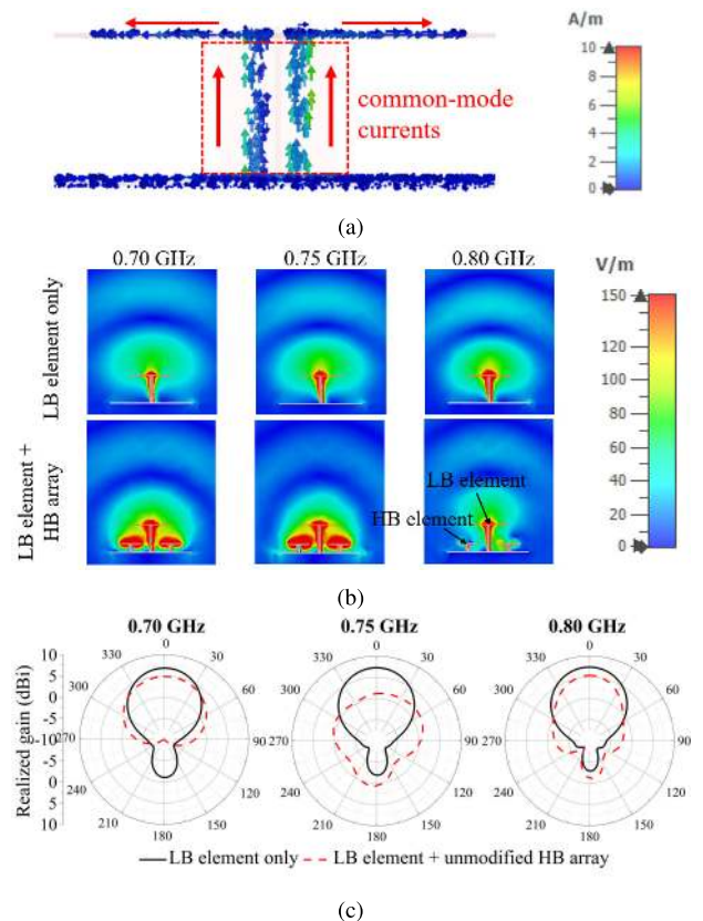
FIGURE 2. (a) The induced LB currents on the HB element at 0.75 GHz. (b) The electric-field distribution, and (c) the horizontal radiation patterns in the low band in the cases of i) only LB element, and ii) LB element with HB array.
