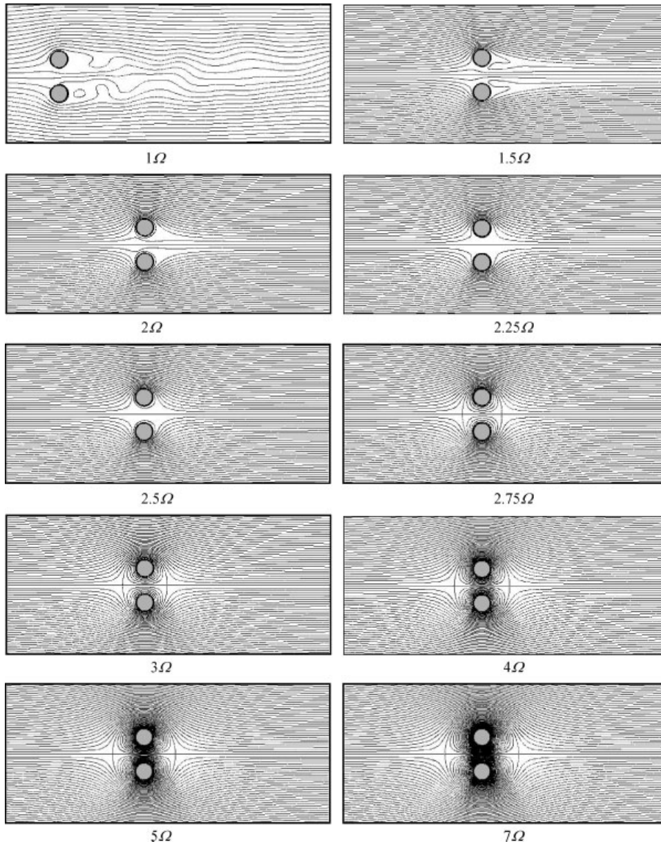
Figure 9. Streamlines showing the evolution of steady flow with increasing rotational speeds, Re_d=150 , g=1 . (Unsteady flow: 1\Omega ; Steady flow: 1.5\Omega , 2\Omega , 2.25\Omega , 2.5\Omega , 2.75\Omega , 3\Omega , 4\Omega , 5\Omega and 7\Omega ).
