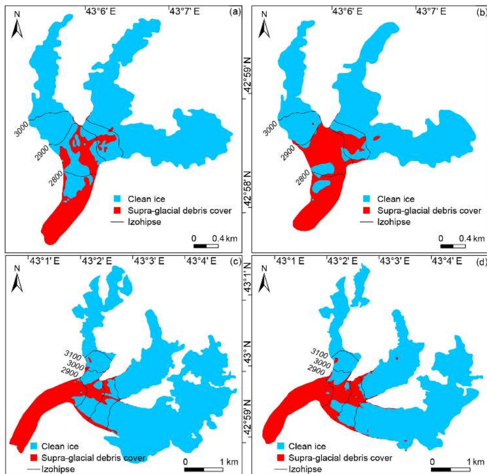
Figure 8. An example of the supra-glacial debris cover up-glacier migration onto Shkhara Glacier in (a) 1986 and (b) 2014 and onto Khalde Glacier in (c) 1986 and (d) 2014.
