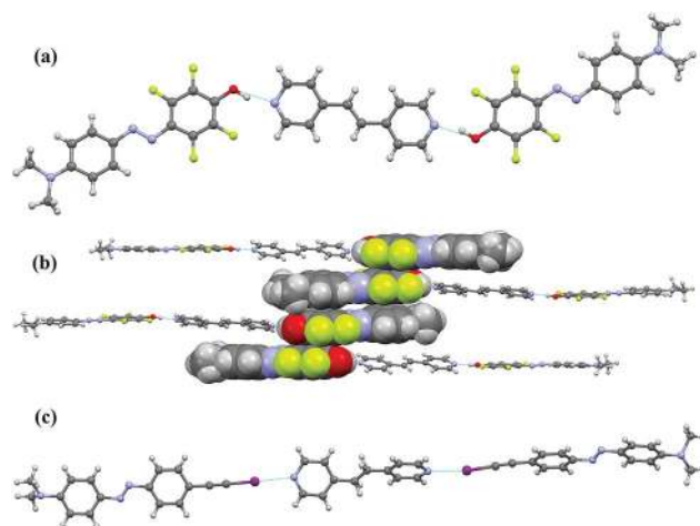
Fig. 3 (a) Ball-and-stick representation of a 10 \cdot (5)_2 hydrogen-bonded trimer. The diazo-molecule is disordered by rotation of 180^\circ around the O...N (amino) axis and only one of the two models is shown. (b) View along the crystallographic b -axis of four 10 \cdot (5)_2 trimers. Four molecules of compound 5, giving strong quadrupolar interactions, are shown in a spacefill style. (c) Ball-and-stick representation of a 10 \cdot (8)_2 halogen-bonded trimer. Both halogen-bond donor and acceptor are heavily disordered over two positions and here only one of the two models is represented. Hydrogen and halogen bonds are pictured as blue dotted lines. Colour code: carbon, grey; hydrogen, white; oxygen, red; nitrogen, blue; fluorine, green and iodine, purple.
