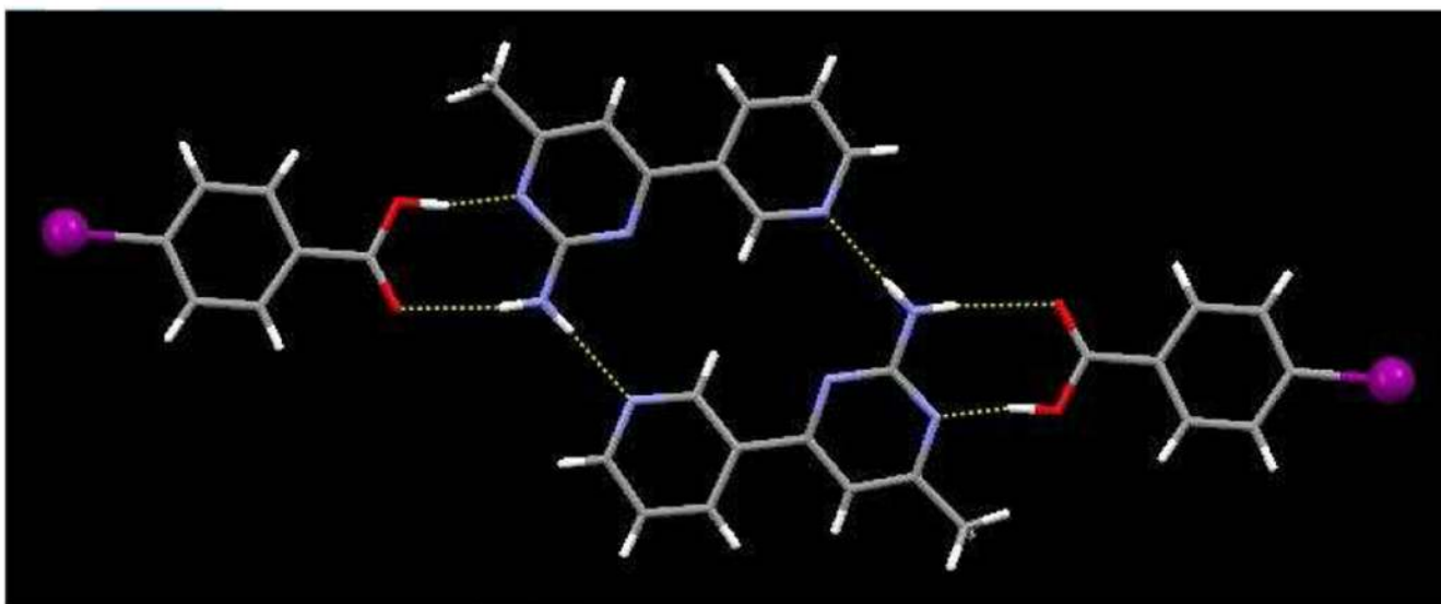
Figure 2. Four-component supermolecule in 1a comprised of N-H...O, O-H...N, and N-H...N hydrogen bonds. The toluene solvent molecule has been omitted for clarity.
