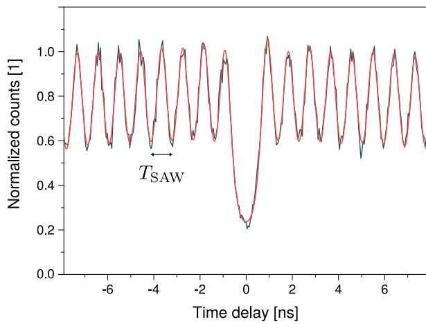
FIG. 4. Second order autocorrelation measurement under cw resonant excitation. A continuous SAW is applied such that the blue extreme of the modulation overlaps with the laser and the cavity. The pulsed curve reflects the SAW modulation period and shows anti-bunching at zero delay. The red line is a cumulative Voigt peak fit with a fixed width.
