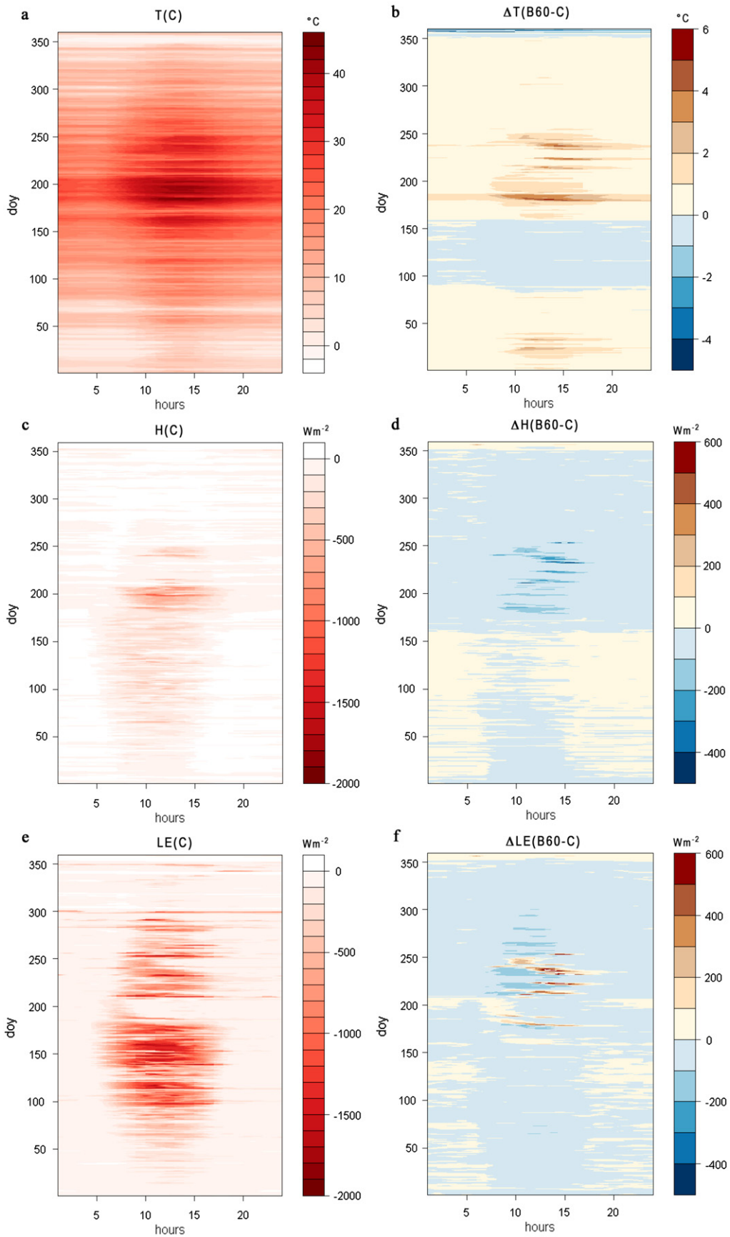
Figure 3. Simulated diurnal cycle of soil surface temperature ( T ) in ^{\circ}\text{C} , sensible ( H ) and latent heat ( LE ) fluxes in \text{W m}^{-2} for control plots ( C ) ((a), (c), (e)) and differences between B60 and control plots (B60-C) ((b), (d), (f)) during year 2010.
