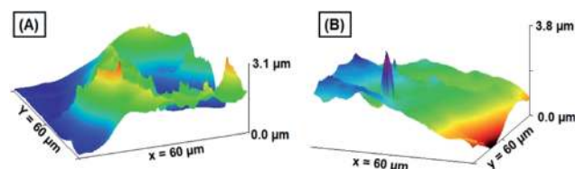
Fig. 7 AFM images of the GNB-modified-ITO electrode (A) before and (B) after the determination of \text{Ce}^{3+} by CV analysis in ABS (pH 4.0 \pm 0.05) at a scan rate of 50 \text{ mV s}^{-1} . Amplitude, spatial, and hybrid details can be found in Fig. S19.†
