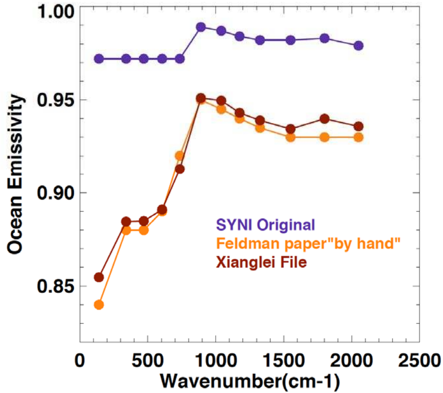
Ocean LW Emissivity in FuLiou Bands
