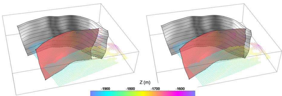
Fig. 9 Defining and enforcing a contact between faults. In this example, the slip is evaluated from the offset of neighboring horizon data (displayed with colored elevation Z ). The contact between the initial red fault and the grey fault is highlighted by red lines (left). After interpolation, the red fault is extrapolated onto the main fault (right)
