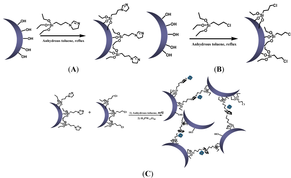
Scheme 1. Typical preparation procedure of the catalysts PW( x )/SiO 2 Im + Cl - SiO 2 . (A) Synthesis of SiO 2 -Im; (B) Synthesis of SiO 2 -Cl; (C) Synthesis of PW( x )/SiO 2 Im + Cl - SiO 2 .
