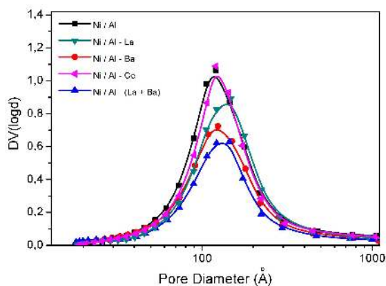
Figure 3. Pore size distributions of the catalysts studied.
