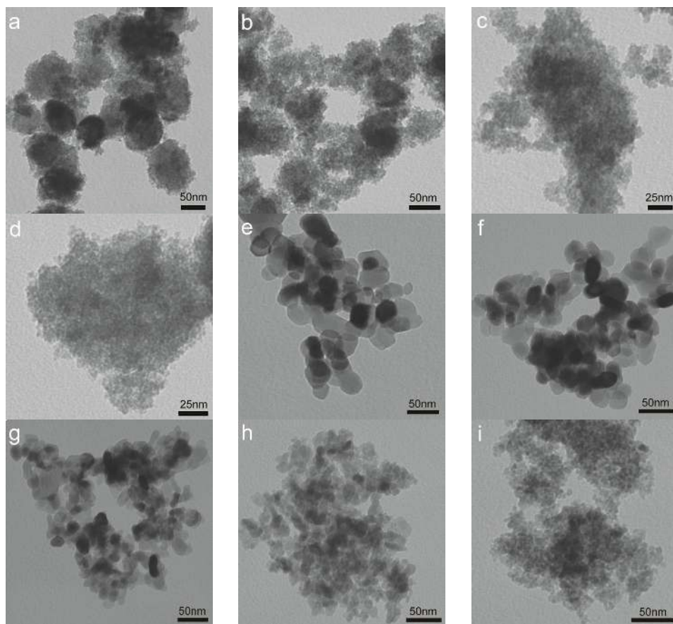
Figure 2. TEM images of fresh Au/FeO x catalysts: (a) Au/Fe 2 O 3 _11.2; (b) Au/Fe 2 O 3 _9.7; (c) Au/Fe 2 O 3 _8.2; (d) Au/Fe 2 O 3 _6.7; (e) Au/Fe 2 O 3 _600; (f) Au/Fe 2 O 3 _500; (g) Au/Fe 2 O 3 _400; (h) Au/Fe 2 O 3 _300; and (i) Au/Fe 2 O 3 _200.
