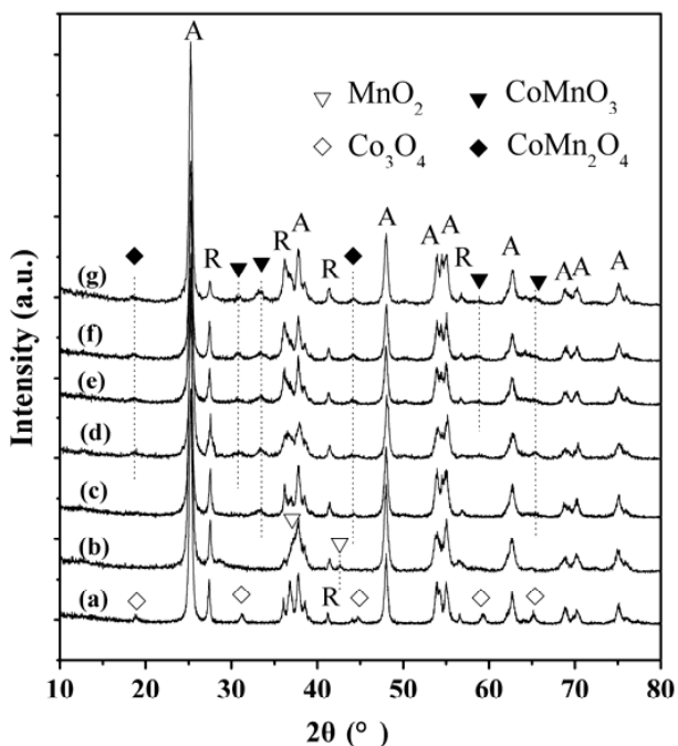
Figure 3. XRD patterns of the catalysts \text{Mn-Co}/\text{TiO}_2 (773 K) with different Co contents: (a) 10\text{Co}/\text{TiO}_2 ; (b) 10\text{Mn}/\text{TiO}_2 ; (c) 10\text{Mn-2Co}/\text{TiO}_2 ; (d) 10\text{Mn-5Co}/\text{TiO}_2 ; (e) 10\text{Mn-8Co}/\text{TiO}_2 ; (f) 10\text{Mn-10Co}/\text{TiO}_2 ; and (g) 20\text{Mn-10Co}/\text{TiO}_2 . (A = anatase phase of \text{TiO}_2 , R = rutile phase of \text{TiO}_2 ).
