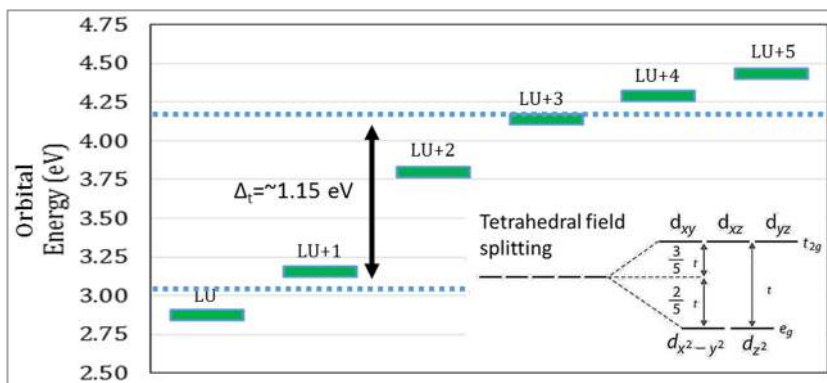
Figure 3. (Left) Energies of selected orbitals and (Right) orbital energies for LU through LU+5. Plotting these orbitals indicated d -orbital character. LU+4 and LU+5 maintain d character but show a signature of orbital mixing, which is why there are a total of six d -like orbitals. A gap in energy exists between LU+1 and LU+2, indicating tetrahedral field splitting. Right inset: expected tetrahedral crystal field d -orbital splitting.
