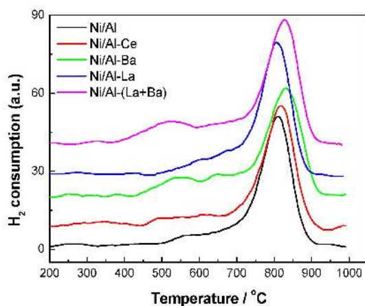
Figure 6. TPR profiles of the prepared catalysts recorded in the temperature range 150–1000 °C.
