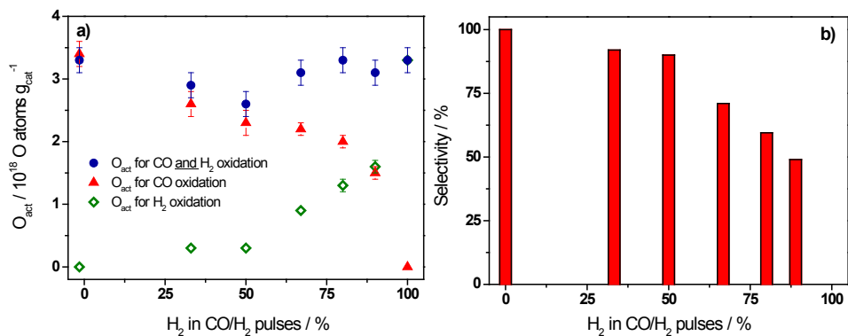
Figure 2. (a) Absolute amounts of active oxygen ( O_{act} ) removal from a fully oxidized Au/TiO 2 catalyst (after O 2 /Ar pulses) by CO and/or H 2 during CO, H 2 , and CO/H 2 pulses with varying ratios of H 2 (33%–89% H 2 ) at 80 °C, and (b) corresponding selectivities for CO oxidation/CO 2 formation during the CO/H 2 /Ar pulses at 80 °C.
