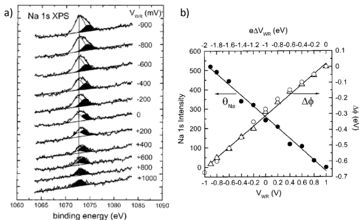
Figure 5. Na 1s XPS spectra taken on a Rh/ \text{Na-}\beta\text{Al}_2\text{O}_3 electrochemical catalyst (580 K, UHV conditions), showing the effect of catalyst potential ( V_{WR} ) on sodium coverage (a). Invariant component due to Na on Rh; shifting component due to Na in solid electrolyte. Influence of V_{WR} on the integrated Na 1s XPS intensity due to Na on the Rh surface and associated work function change of the catalyst film (b). Reprinted with permission from Ref. [41]. Copyright 2000 American Chemical Society.
