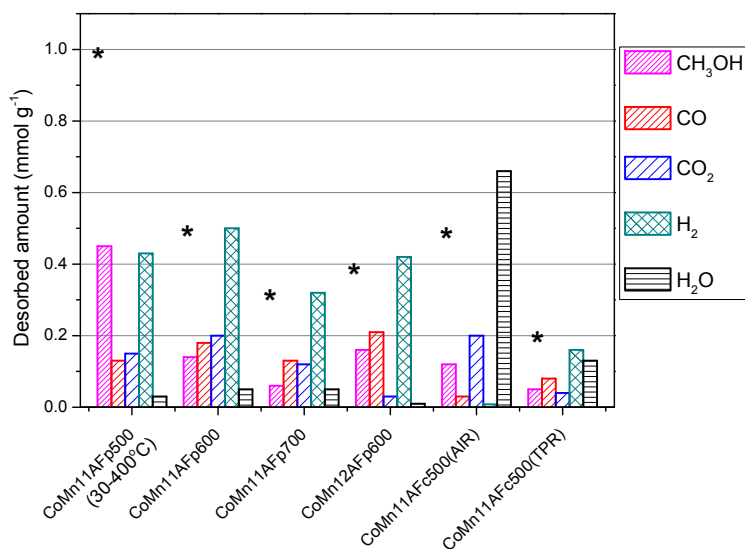
Figure 12. Desorbed amounts of CH 3 OH, CO, CO 2 , H 2 and H 2 O during TPD after CH 3 OH adsorption. Adsorbed amount of methanol is shown with asterisks (*).
