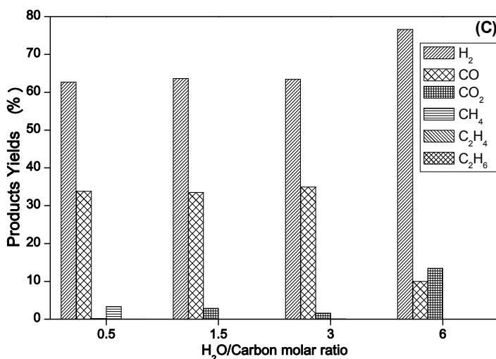
Figure 9. Effect of H 2 O/Carbon (S/C) feed molar ratio on product yield at 400 °C (A); 600 °C (B) and 800 °C (C) over 20 wt.% Co/CeO 2 catalyst. Reaction conditions: m_{\text{cat}} = 250 \text{ mg} , F_T = 150 \text{ cm}^3/\text{min} .
