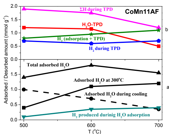
Figure 7. (a) Total adsorbed \text{H}_2\text{O} at 300 ^{\circ}\text{C} and \text{H}_2 produced during water adsorption; and (b) \text{H}_2\text{O} desorbed and \text{H}_2 producing during TPD. \text{CoMn11AF}_i with i = 500, 600, 700 ^{\circ}\text{C} .
