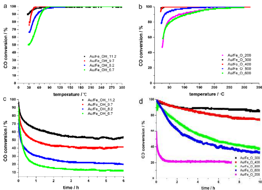
Figure 5. CO conversions of fresh Au/FeO x catalysts for the low-temperature CO oxidation reaction: (a) Au/Fe OH , transient; (b) Au/Fe O , transient; (c) Au/Fe OH , stability at 30 °C; and (d) Au/Fe O , stability at 30 °C. Reaction conditions: 1% CO/20% O 2 /79% N 2 , 80,000 mL·h -1 ·g cat -1 .
