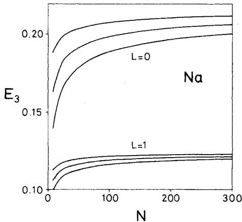
FIG. 5. L=0 (upper curves) and L=1 (lower curves) obtained in the TF approximation using Eq. (41). For each multipolarity, the curves correspond to a=0.72 a.u. (upper), a=1.02 a.u. (middle), and a=1.32 a.u. (lower).
