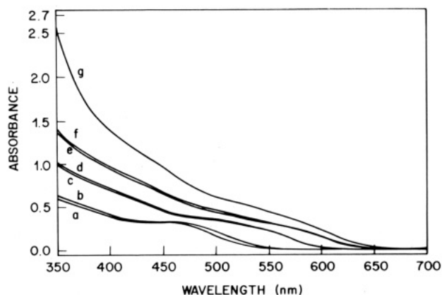
Figure 3. UV-visible spectra of the CdSe growth experiment. Traces a through f are in the heptane/AOT/ \text{H}_2\text{O} reaction medium, with the starting cadmium-containing solution as the reference. Trace g is in pyridine with pure pyridine as reference. After addition of (a) 44 \mu\text{mol} of \text{Se}(\text{TMS})_2 to the initial \text{Cd}^{2+} solution (see text); (b) 30 \mu\text{mol} of \text{Cd}^{2+} (as a micellar solution); (c) 20 \mu\text{mol} of \text{Se}(\text{TMS})_2 ; (d) 30 \mu\text{mol} of \text{Cd}^{2+} ; (e) 30 \mu\text{mol} of \text{Se}(\text{TMS})_2 ; (f) 60 \mu\text{mol} of \text{Cd}^{2+} . (g) Spectrum of capped CdSe molecular particles after isolation, washing, and redissolution in pyridine.
