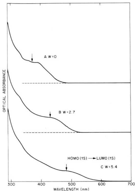
Figure 1. Optical absorption spectra (25 °C) of CdSe clusters synthesized and stabilized in microemulsion media. Synthesis conditions: [AOT] = 0.05 M, [\text{Cd}(\text{ClO}_4)_2] = 7.5 \times 10^{-4} M, [\text{Se}(\text{TMS})_2] = 5 \times 10^{-4} M; (A) W = 0 ; (B) W = 2.7 ; (C) W = 5.4 . The lowest, size dependent HOMO \rightarrow LUMO transition is marked with an arrow in each case. The curves are offset vertically for clarity.
