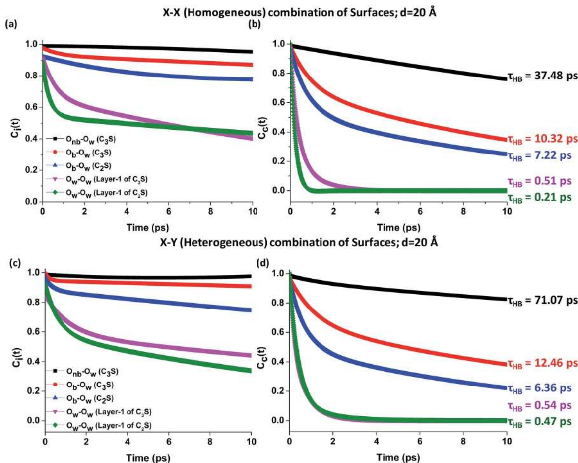
Fig. 9 Hydrogen bond dynamics for various donor-acceptor pairs with homogeneous and heterogeneous surface combinations. (a) Interrupted and (b) continuous H-bond autocorrelation function on homogenous/similar C 3 S-C 3 S and C 2 S-C 2 S surface combination at a surface separation of d = 20 \text{ \AA} (c) interrupted and (d) continuous H-bond autocorrelation function on heterogeneous/dissimilar C 3 S-C 2 S surface combination at a surface separation of d = 20 \text{ \AA} . All possible donor-acceptor combinations are considered.
