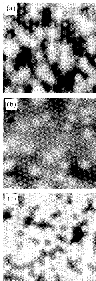
FIG. 1. (a) 100\times 80\text{-}\text{\AA}^2 tunneling image showing the ( \sqrt{3}\times\sqrt{3} )R30° structure after annealing degenerately boron-doped Si(111) at 1000°C. Tip bias = -1.4 V, 1 nA. (b) 100\times 100\text{-}\text{\AA}^2 tunneling image of Si(111) prepared by sputtering of B on clean Si(111)7×7. (c) 100\times 100\text{-}\text{\AA}^2 tunneling image prepared by Si reevaporation on Si(111)( \sqrt{3}\times\sqrt{3} )R30°-B.
