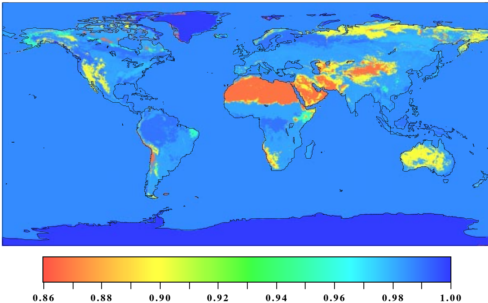
Figure 6. CERES Window (8-12 \mu\text{m} ) Surface Emissivity on 10' grid
