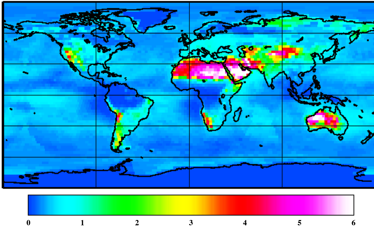
Figure 9: Difference in NLW Flux ( \text{Wm}^{-2} ) : Flux with variable \epsilon - flux with constant \epsilon
