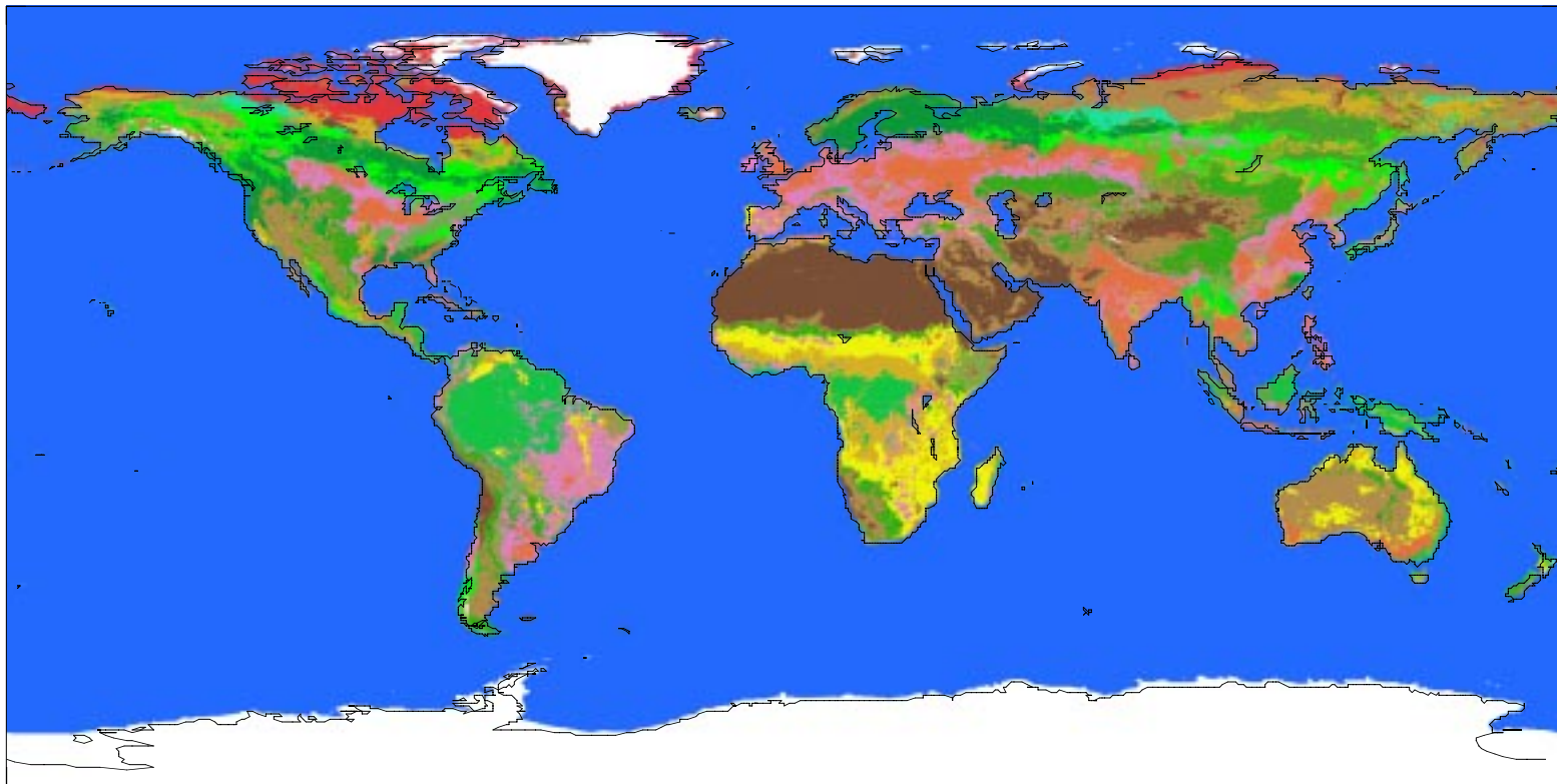
Figure 3. Surface Types on 10' grid.
