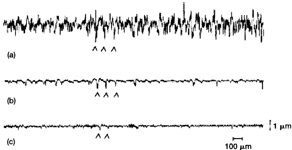
Figure 5.—Typical relocated surface features measured using a profilometer followed by filtering of the data using a 0.08-mm (0.003-in.) cutoff. Evidence of persistence of the deepest grinding marks are indicated by arrows. (a) Ground tooth surface, R_a = 0.434 \mu\text{m} (17 \mu\text{in.} ). (b) Same tooth surface after the first stage of superfinishing, R_a = 0.083 \mu\text{m} (3.3 \mu\text{in.} ). (c) Same tooth after second (final) stage of superfinishing, R_a = 0.056 \mu\text{m} (2.2 \mu\text{in.} ).
