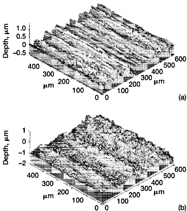
Figure 6.—Comparison of tooth gear surface topographies as measured using a mapping interferometric microscope. (a) Ground gear tooth. (b) Superfinished gear tooth.
