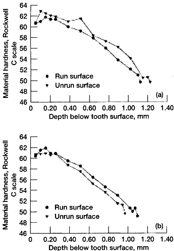
Figure 3.—Material hardness versus depth below the pitch radius surface. (a) Superfinished gear. (b) Ground gear.
