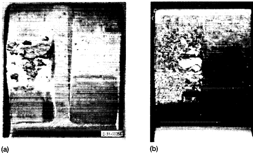
Figure 7.—Typical fatigue damage. (a) Ground gear. (b) Superfinished gear.
