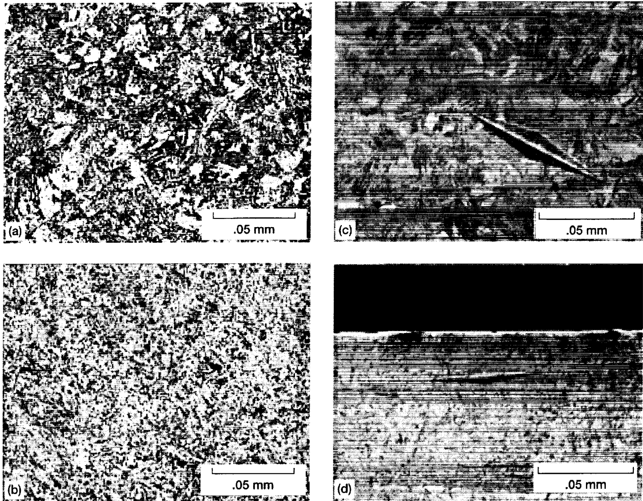
Figure 2.—Microphotographs of the gears prepared with 3% nital etch. (a) Core of superfinished gear. (b) Case of superfinished gear. (c) Core of ground gear. (d) Case of ground gear.
