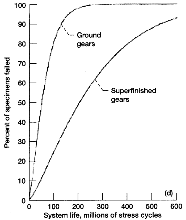
Figure 8.—Surface fatigue lives on ground and superfinished AISI 9310 gear pairs. (a) Ground gears. (b) Superfinished gears. (c) Summary of linear least-squares-fit lines. (d) Linear least-squares-fit lines plotted on linear axes.
