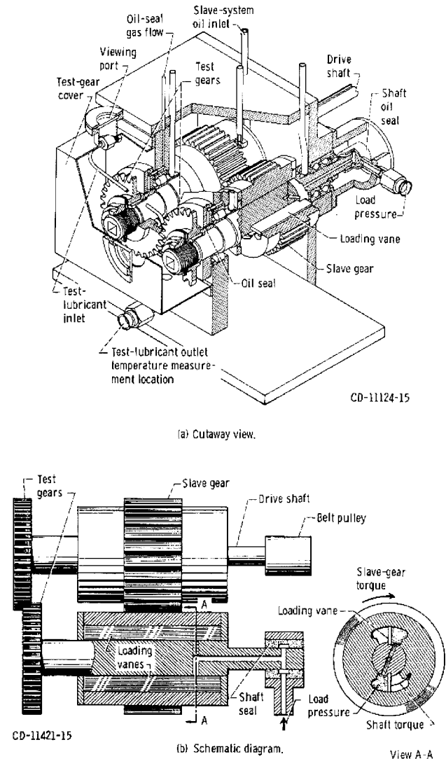
Fig. 1 NASA Glenn Research Center gear fatigue test apparatus: (a) cutaway view; (b) schematic view.
