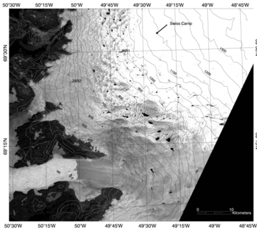
Fig. 1. Elevation contours (50 m) on a Landsat Thematic Mapper image (channel 3) taken on 22 June 1990, which is typically about one-third of the way through the melt season. Locations of the Swiss Camp and the Automated Weather Station at JAR-1 and JAR-2 are marked. The indicated flowline direction of 235^{\circ}\text{E} at the camp curves westward toward the grounded ice edge. The grayer areas at lower elevations in the image are bare ice, with some whiter patches of remaining winter snow near the ice-snow line. By the end of the melt season in late August to early September, the firn-ice boundary usually retreats to around the average location of the equilibrium line ( 15 ) near the Swiss Camp. The dark patches are melt lakes, some of which show dark lines of inflow channels. Later in the season, melt lakes also form above the equilibrium line. Jacobshavn Isbrae is in the lower part.
