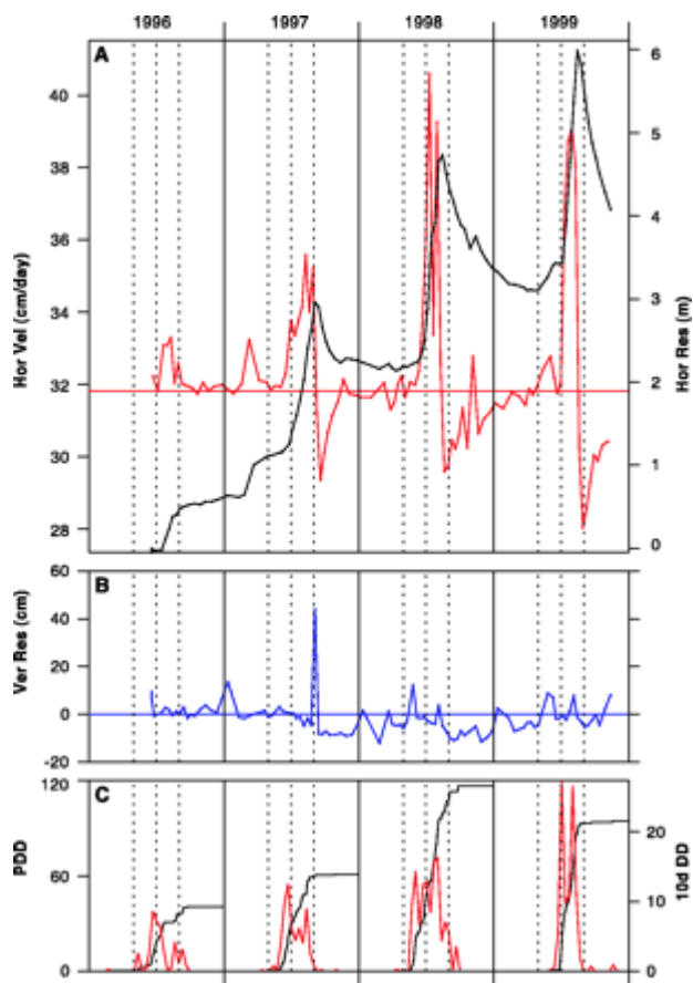
Figure 3. (A) Horizontal ice velocity (red curve) along a smoothed line of motion showing ice accelerations during the summer melt seasons and the abrupt transitions to deceleration around the times of melt cessation. The cumulative additional motion (horizontal residual, black) relative to a wintertime-average velocity of 31.33 cm/day is 6.0 m by the time of the maximum velocity in 1999. (B) The vertical residual (blue) indicates a 50-cm uplift at the time of the 1997 transition from accelerating flow to decelerating flow. (C) Cumulative PDDs and PDDs for 10-day intervals (10d DD, red) from temperatures measured at the Swiss Camp, showing correlations of the melting with the intensity and timing of the ice accelerations and decelerations (units are degree-days). Vertical dotted lines mark May 1, July 1, and September 1 for each year.
