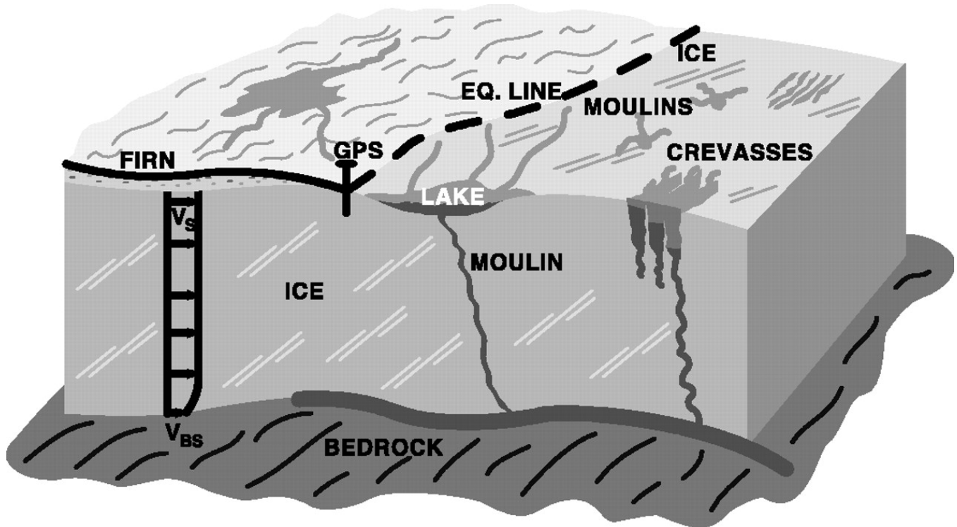
Fig. 2. Schematic of glaciological features in the equilibrium and ablation zones, including surface lakes, inflow channels, crevasses, and moulin. Ice flow for basal ice at the pressure melting point is partly from basal sliding and partly from shear deformation, which is mostly in a near-basal boundary layer.
