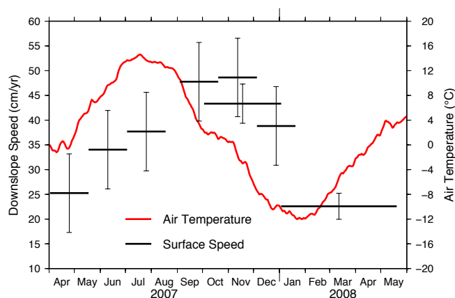
Fig. 6. Time series of the smoothed air temperature (red line) and the InSAR-estimated downslope speed (horizontal bars) at the marker “A” shown in Fig. 5b. The extent of each horizontal bar represents the period from which the speed is estimated (see Sect. 3.1). The vertical error bars are the 1\sigma uncertainties of the measured speed.
