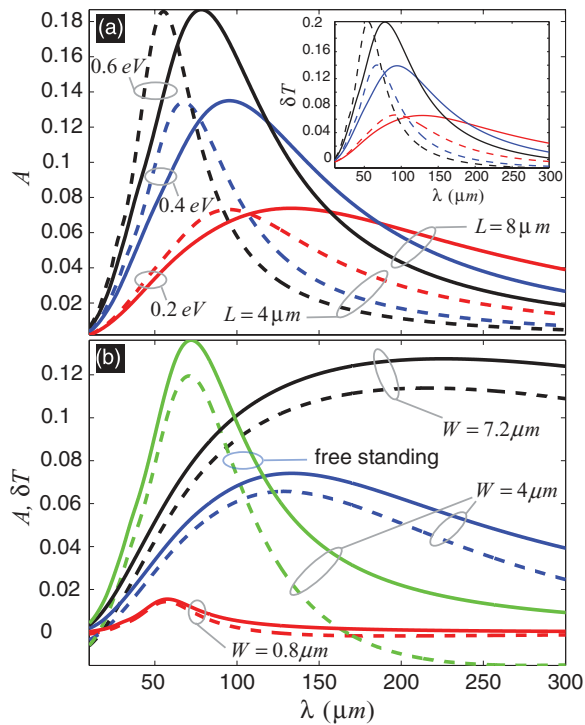
FIG. 2. (Color online) Absorption and gate-induced change of transmission spectra for PAGR with the dielectric cladding and relaxation time corresponding to the experiment in Ref. 21: \varepsilon_1 = 3 , \varepsilon_2 = 4 , \tau = 0.25 ps. (a) shows the absorption spectra A for different values of chemical potential \mu . The continuous curves are for the period L = 8 \mu\text{m} , while the discontinuous ones are for L = 4 \mu\text{m} . For both cases W = L/2 . In the inset the relative change of transmission with respect to the sample at charge neutral point \delta T = -(T - T_{\text{CNP}})/T_{\text{CNP}} is shown for the same L and W as in the main figure. In (b) the spectra for A (continuous curves) and \delta T (discontinuous curves) are shown for different widths of the ribbons W for L = 8 \mu\text{m} , \mu = 0.2 eV. The case of W = 4 \mu\text{m} is also shown for the freestanding graphene ( \varepsilon_1 = \varepsilon_2 = 1 ).
