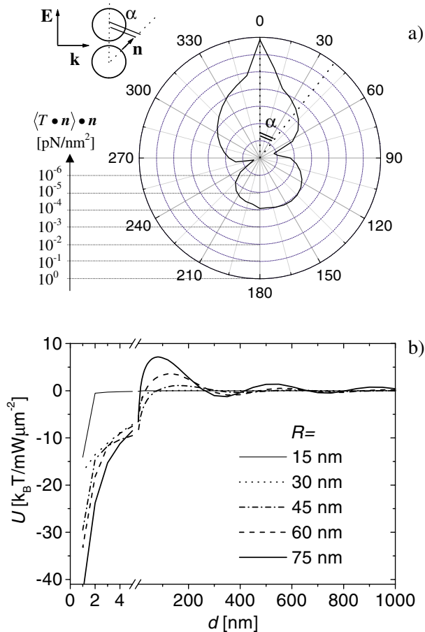
FIG. 4 (color online). (a) Polar plot of the optical force per area unit, ^{10}\log(\langle \mathbf{T} \cdot \mathbf{n} \rangle \cdot \mathbf{n}) , for the lower particle in a dimer (see inset, I_0 = 1 \text{ mW}/\mu\text{m}^2 , \lambda = 514.5 \text{ nm} , R = 45 \text{ nm} , d = 1 \text{ nm} ); (b) interparticle optical potential U(d, R) for dimers in water ( T = 300 \text{ K} , polarization configuration shown in inset).
