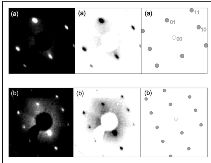
Figure 3. (1×1) LEED patterns (left) recorded using beam energies of (a) 31 eV and (b) 49 eV from InAs(110) prepared by an AHC dose of 120 kL with a sample temperature of 400°C. The inverted images (centre) and schematic diagrams (right) are also shown. The diffraction spots obscured by the electron gun are shown unshaded in the schematic pattern.
