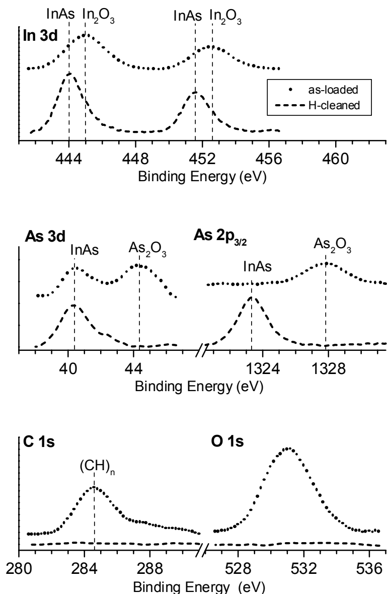
Figure 1. In 3d, As 3d, As 2p 3/2 , C 1s and O 1s XPS spectra from as-loaded InAs(110) (dotted lines) and from clean InAs(110) prepared by an AHC dose of 120 kL with a sample temperature of 400°C (dashed lines). All y-axes are in arbitrary units.
