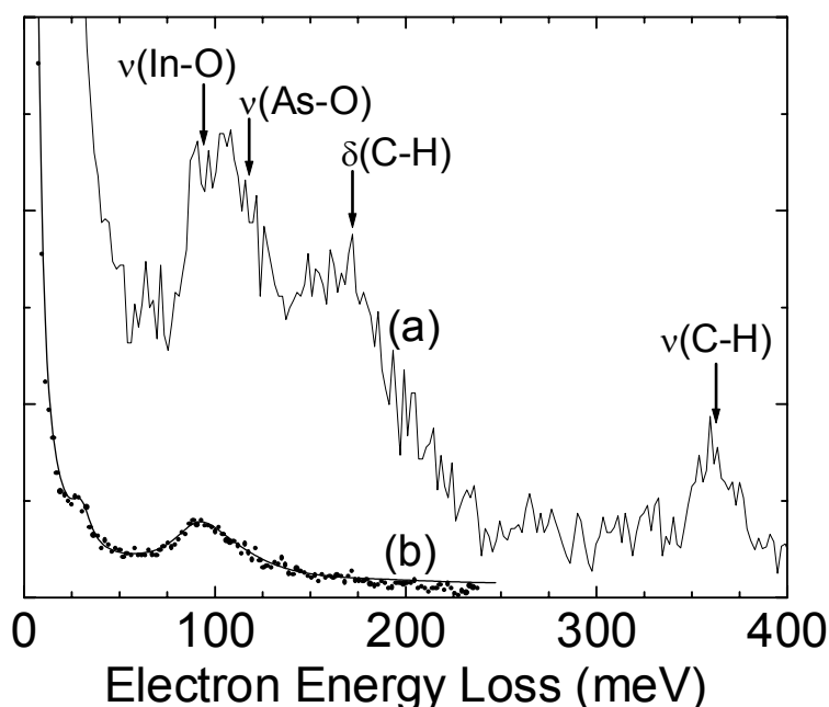
Figure 2. Specular HREEL spectra, recorded at 15 eV, with an instrumental broadening of 10 meV FWHM, from (a) an as-loaded InAs(110) sample; (b) after annealing for one hour at 360^\circ\text{C} and a total of 120kL of atomic hydrogen cleaning at a sample temperature of 400^\circ\text{C} . The dotted line of spectrum (b) depicts the experimental points and the solid line is the simulated spectrum calculated using semi-classical dielectric theory.
