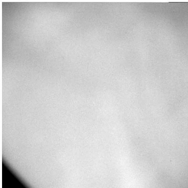
Figure 7. Ratio of dark-corrected sky flat taken with dust cover closed to dark-corrected sky flat taken with dust cover open. Both images acquired on sol 90. The vignetting at lower left is caused by black tape that was added to the MI dust cover to allow verification of cover state based on image data.
