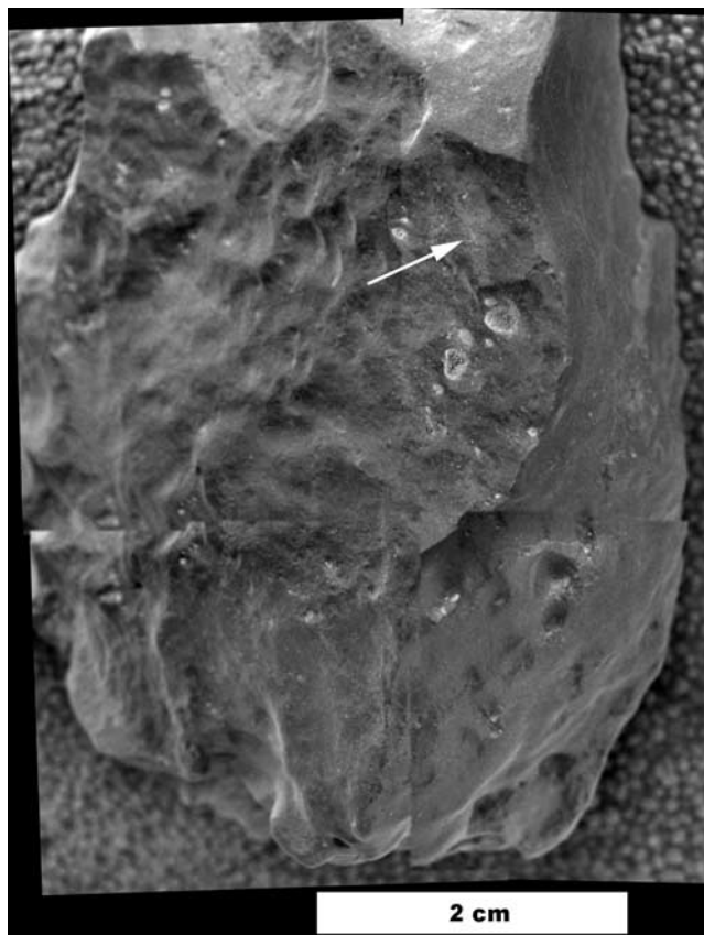
Figure 27. MI mosaic of cobble Antistasi, taken on sol 641 when fully shadowed. Cobble reflectance is heterogeneous, with irregular lighter areas (arrow) embedded in a darker mass.
