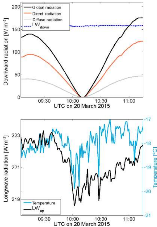
Figure 5. The downward radiation components' shortwave direct, diffuse, and global radiation as well as downward thermal radiation ( \text{LW}_{\text{down}} ) and 2 m temperature ( \text{LW}_{\text{up}} ) between 09:10 and 11:10 UTC on 20 March 2015 in Ny-Ålesund.
