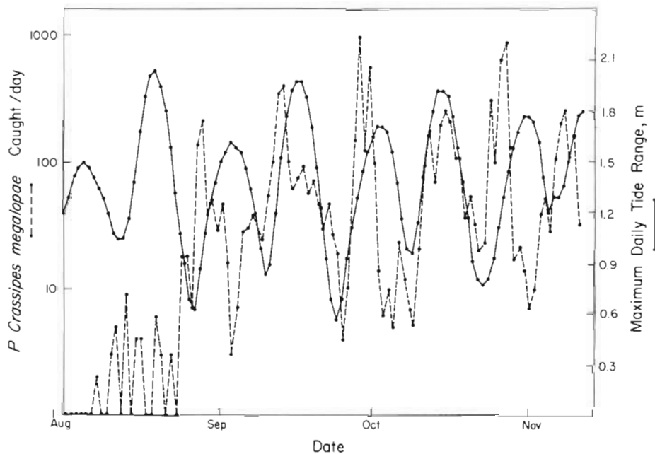
Fig. 1. Pachygrapsus crassipes . Log of daily catch of megalopa larvae from traps (0 m plus 1.5 m) hung under the lights at the end of Scripps pier (dashed line) plotted against maximum tidal range per 24 h period (solid line)
