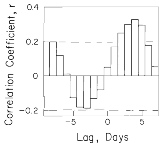
Fig. 2. Pachygrapsus crassipes . Cross correlation of daily catch of megalopa larvae vs. maximum daily tidal range. Cross correlation was limited to lags of \pm 8 d. 10% of record length (Otnes and Enochson, 1978). Critical r = 0.217 for P < 0.05 and n = 80
