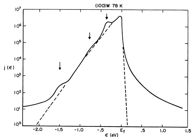
FIG. 1. Total energy distribution of field emitted electrons from (100) plane of tungsten. The dashed lines indicate a free-electron energy distribution by Eq. (1). The ordinate represents the counts per 0.020 \text{ eV} .
