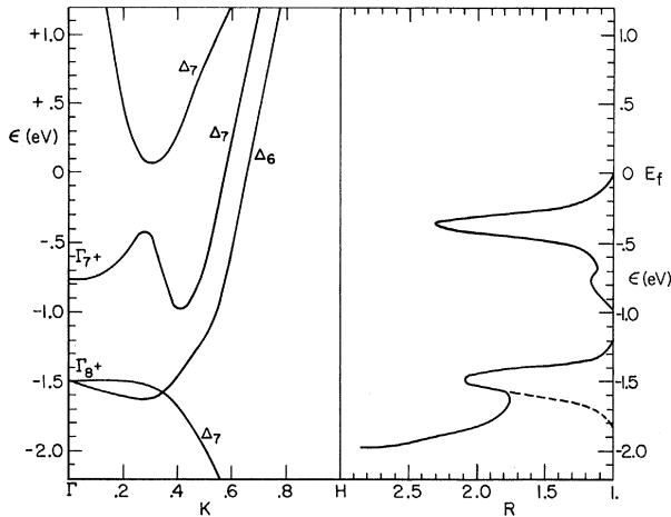
FIG. 2. (a) Relativistic energy bands for the (100) direction of tungsten calculated by Loucks (Ref. 5), showing the two gaps created by the splitting of the three \Delta_7 bands. (b) The experimental enhancement factor R(\epsilon) for the (100) plane of tungsten [defined in Eq. (2)].
