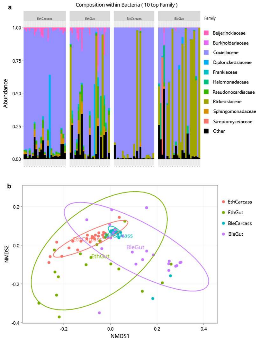
Fig. 2 Effect of the sterilization treatment on the internal microbiome of ticks. a Bar plots of the relative abundance of the 10 most abundant bacterial families in each sample regrouped by sample categories; EthCarcass corresponds to ethanol-treated carcass ticks, EthGut to ethanol midguts, BleCarcass to bleached carcass ticks, and BleGut to bleached tick midguts. b NMDS plot of generalized Unifrac ( \alpha=0.5 ) distances between all categories with ellipses encompassing normal confidence range for each category
