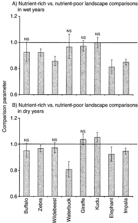
FIG. 8. Comparison parameter estimates, c_{kl} (see Methods: Data analyses for details), are plotted to summarize differences between species' distance-to-water distributions in the nutrient-rich vs. nutrient-poor landscape; c_{kl} values are calculated for both the (A) wet-year and (B) dry-year data subsets (NS indicates comparisons that are not significant at a 95% family confidence level). Values of c_{kl} < 1 imply that the probability of a herd's presence falls more steeply as distance to water increases (i.e., herds are more likely to occur close to water sources) in the nutrient-rich compared to nutrient-poor landscape.
