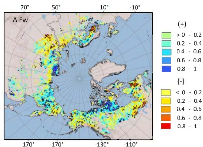
Figure 5. Recent summer AMSR-E Fw wetting and drying trends in the northern ( >45^\circ N) wetland regions, indicated by Mann-Kendall tau rank coefficients. Positive (negative) tau represents an increase (decrease) in surface water cover. Black polylines denote areas having significant ( p<0.05 , |\text{tau}|>0.6 ) change in surface water extent over the 2003–11 satellite observation record.
