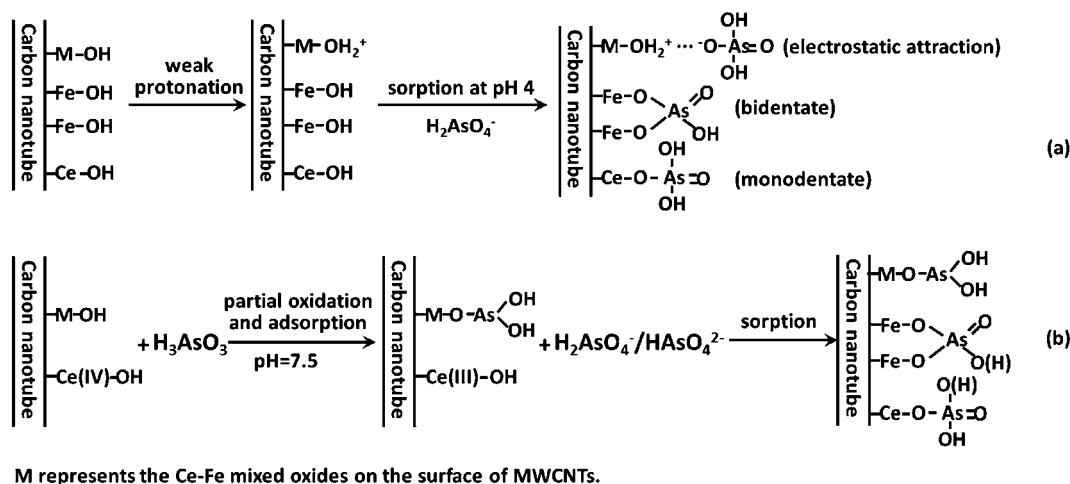
Fig. 13 Schematic diagram for the proposed mechanism of As(v) (a) and As(III) (b) adsorption on CF-CNTs.
