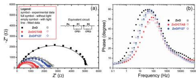
Fig. 12 (a) EIS of the ZnO photoanodes recorded in dark condition and under visible light illumination with the equivalent circuit model as an inset, and (b) Bode phase plots.
