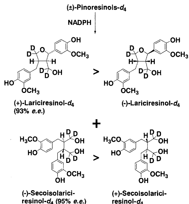
Fig. 3. Enantiomeric compositions of [ ^2H_4 ]lariciresinol and [ ^2H_4 ]secoisolariciresinol formed enzymatically from (±)-[9,9,9',9'- ^2H_4 ]pinoresinols
