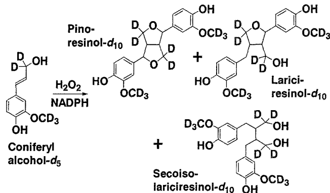
Fig. 2. Enzymatic conversion of [9,9- ^2 H _2 , OC ^2 H _3 ]coniferyl alcohol to [ ^2 H _{10} ]pinosresinol, [ ^2 H _{10} ]lariciresinol, and [ ^2 H _{10} ]secoisolariciresinol
