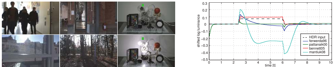
Figure 1: Left: The HDR-video sequences used in our evaluation exhibit strong local contrast changes, rapid variations in local and global intensity as well as spatio-temporal variations. Right: the plot illustrates how different a set of representative TMOs from our evaluation, see legend, responds to the same HDR input. The plot shows the log luminance of the temporal variation of a pixel under the green square as the light bulbs are turned on and off. Note that the plots are, for presentation purposes, shifted along the y-axis to start at the same value.
