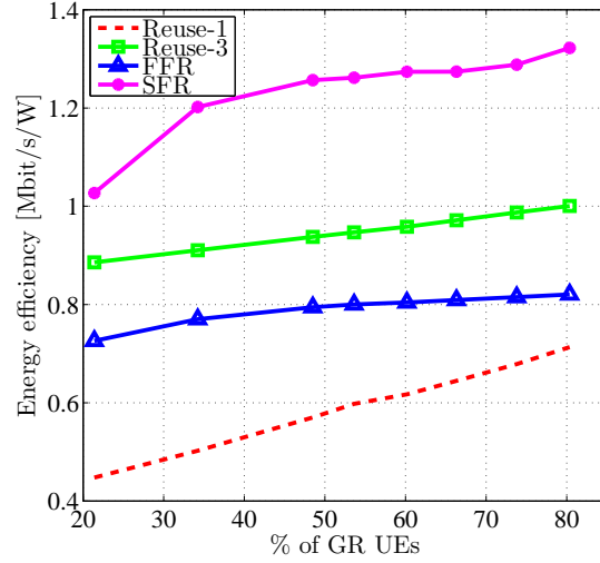
Fig. 13: Energy efficiency versus percentage of GR UEs
