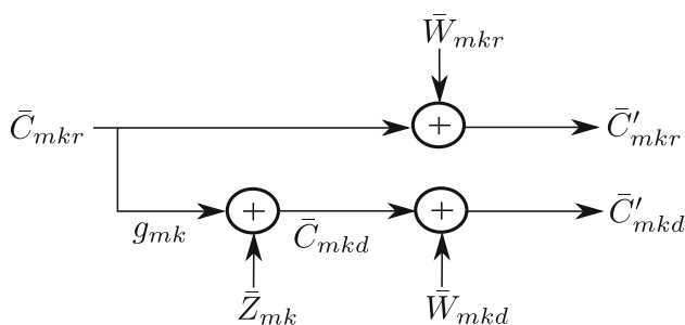
Fig. 1 QA Model for VIF Index
